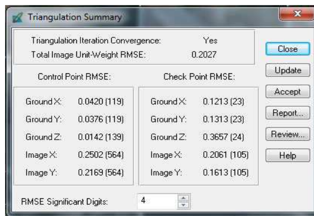
Figure 2. Triangulation summary
